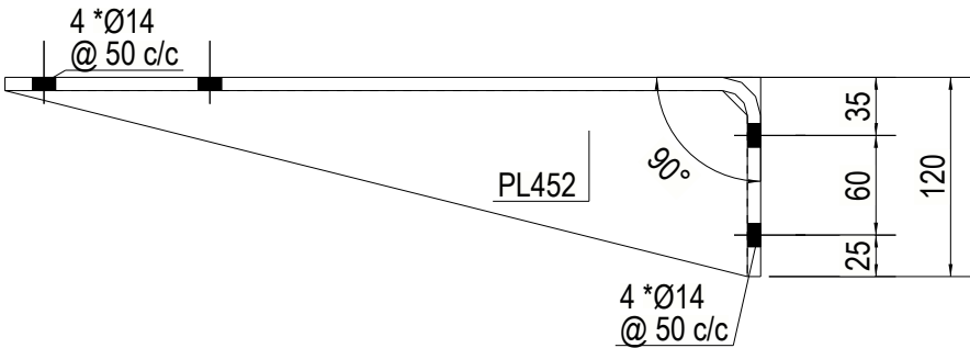
TOP VIEW
